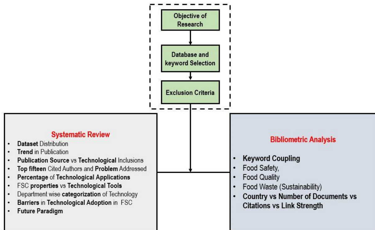
Figure 1. Methodology.
