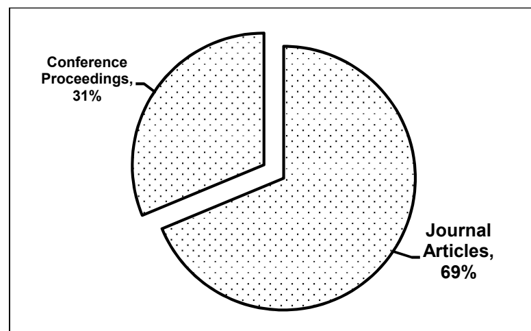
Figure 2. Dataset Distribution.
