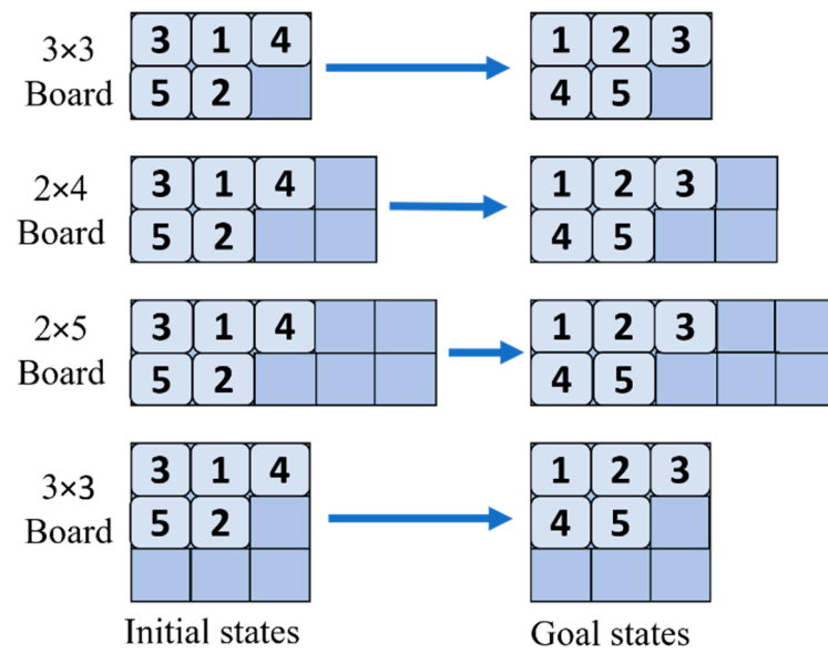
Figure 9. An example of the examination of the same state configurations with different board sizes and shapes.
