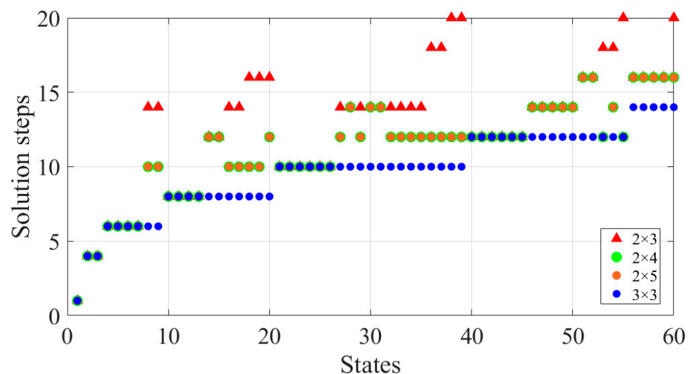
Figure 10. Comparison between different board sizes and shapes for the same number of boxes.
