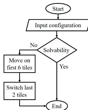
Figure 7. Flowchart of the pre-sorting process.
