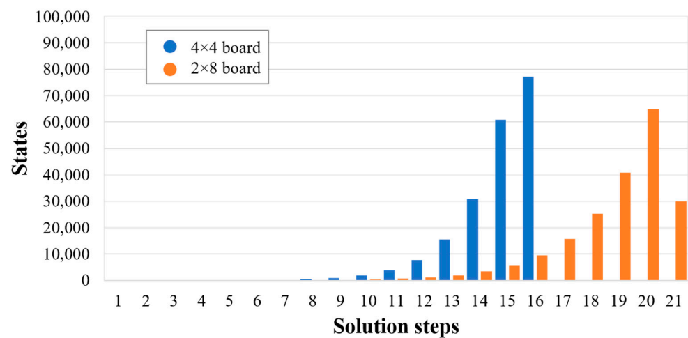
Figure 14. Comparison between the 4 \times 4 and 2 \times 8 board sizes with non-random states regarding the solution steps.
