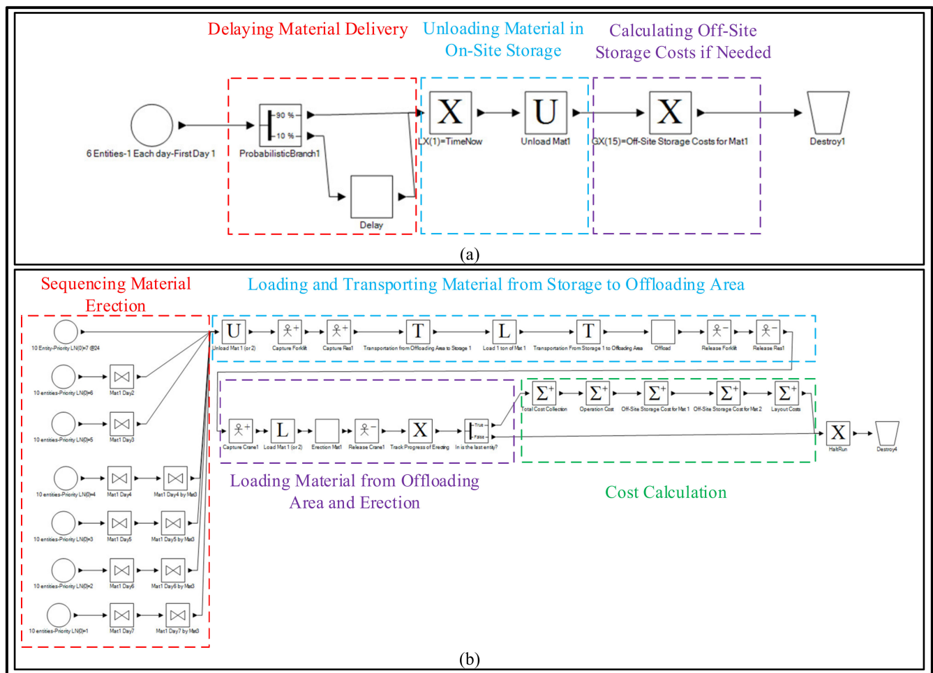
Figure 13. (a) Overview of the simulation model for material delivery and (b) overview of the simulation model for material erection.
