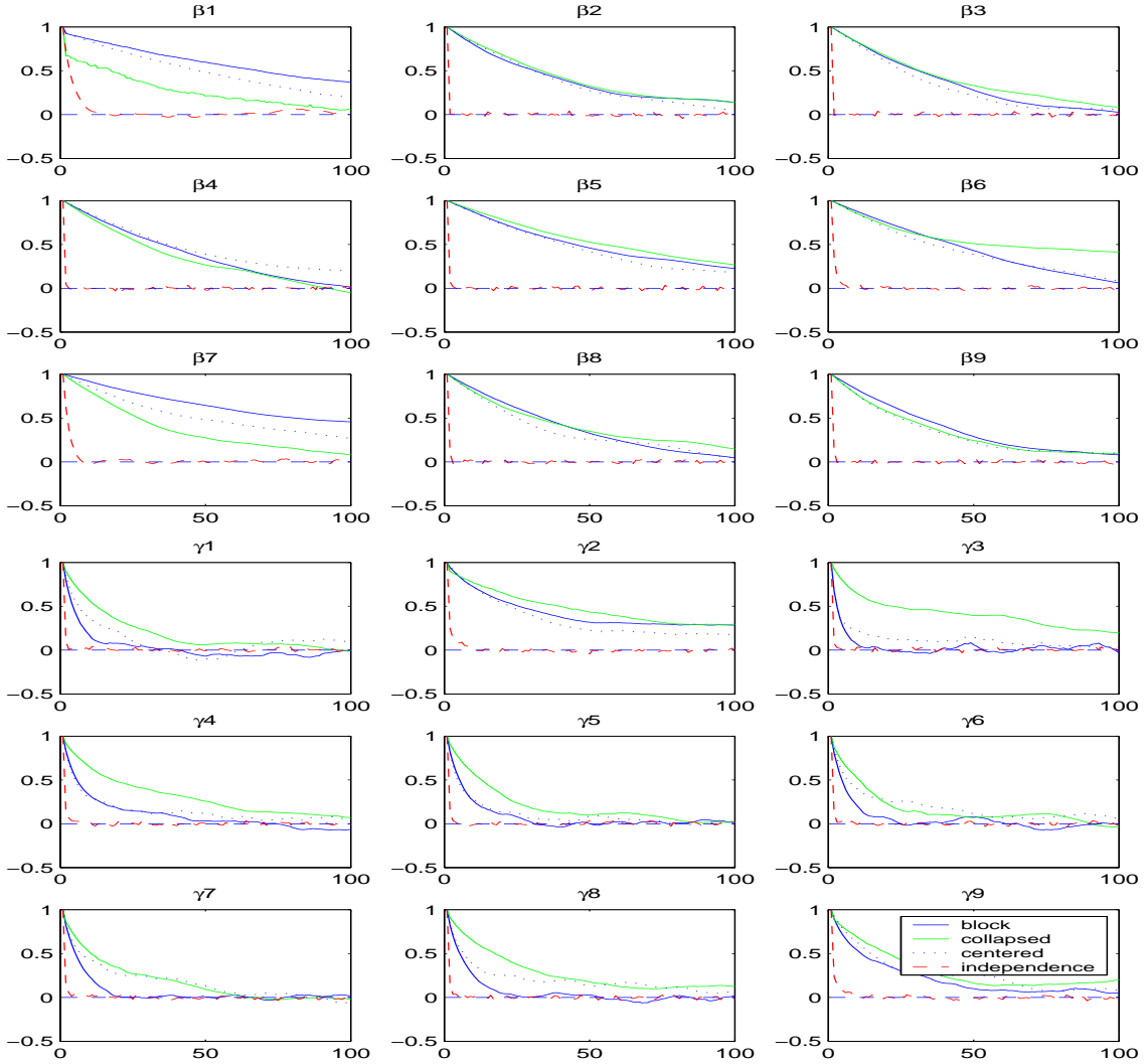
Figure 6: Estimated empirical autocorrelations for \beta(\gamma_1, \dots, \gamma_9) and for the real data set using the block , collapsed , centered and independence update strategies
