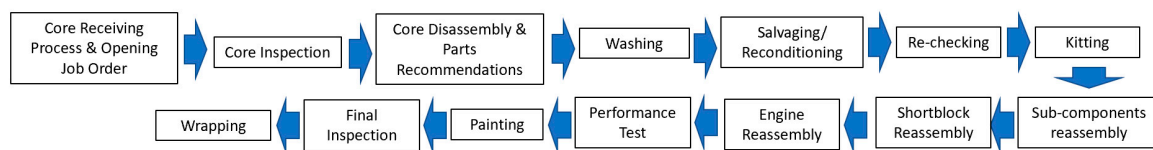
Figure 1. The remanufacturing activities at HeavyEq.
