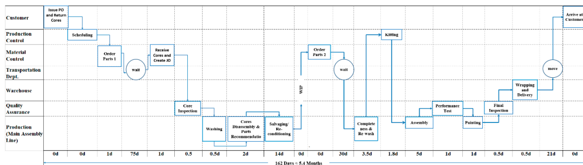
Figure 2. A time function map of the remanufacturing activities.
