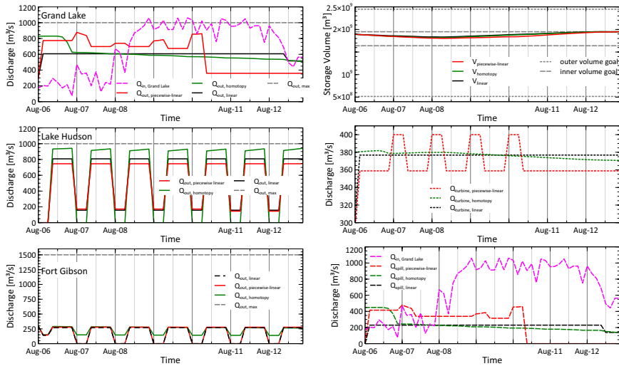
(a) Reservoir release for Grand Lake, Lake Hudson and Fort Gibson (b) Optimization result for volume, spill flow and turbine flow for Grand Lake
