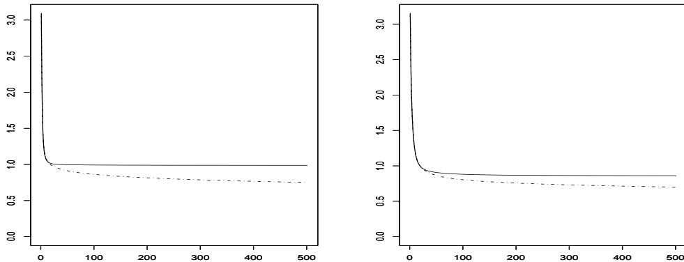
FIGURE 5: \hat{\sigma}^2 vs. the number of boosting iterations, averaged over 50 simulations for MonBoost (solid) and componentwise L2Boost (dotted), piecewise constant (left panel) and plateau (right panel) function with n = 30 and \sigma = 1 with logistic basis functions.
