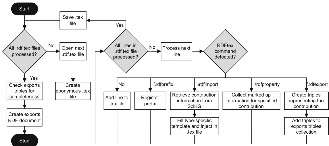
Fig. 5 A flowchart of RDFtex's preprocessing workflow. For conciseness, the injection of custom L A T E X environments, which are necessary for importing some of the supported contribution types, was omitted
