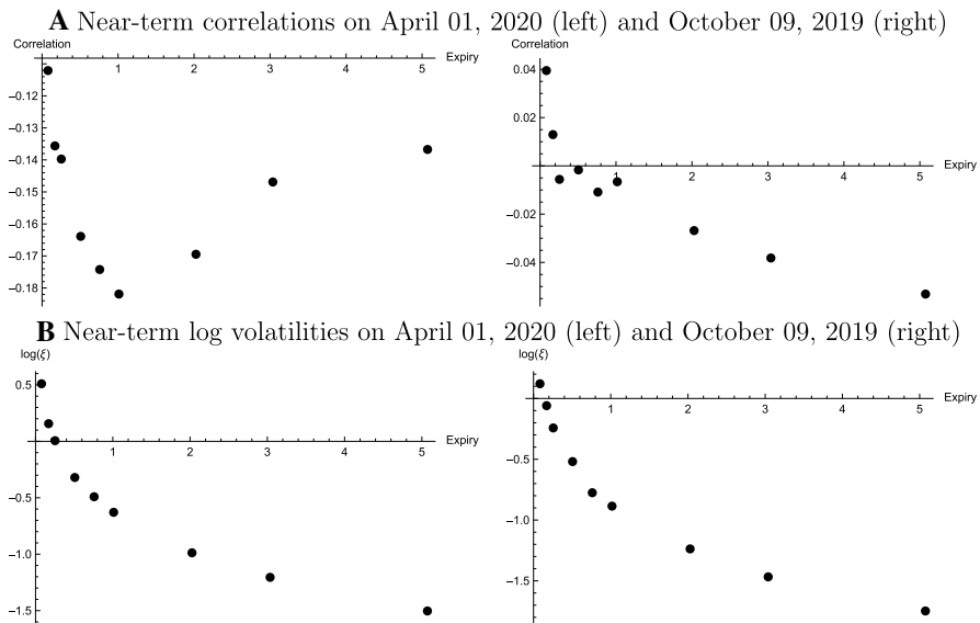
Fig. 3 Calibrated Model Parameters: Arbitrage-Free Approach. The figure shows near-term volatilities of implied volatilities ( \log \xi_t^I ) and near-term correlations ( \rho_t^I ) with respect to option expiry dates. The figures on the left and the right refer to April 01, 2020 and October 09, 2019, respectively
