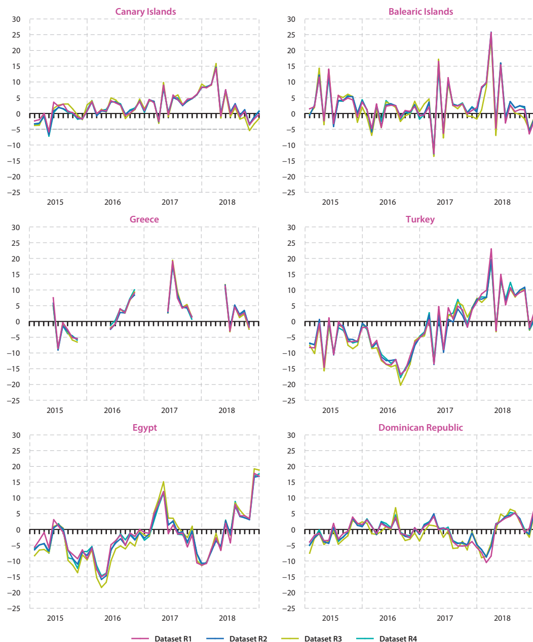
Figure A.3: Comparison of annual rates of change for double imputation using different datasets
