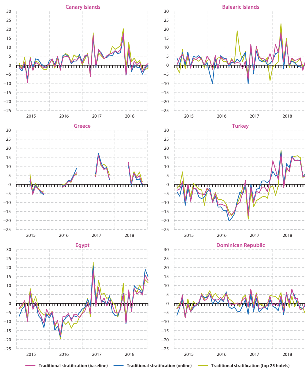
Figure A.4: Comparison of annual rates of change for different versions of traditional stratification (% change compared with same month of the previous year)
