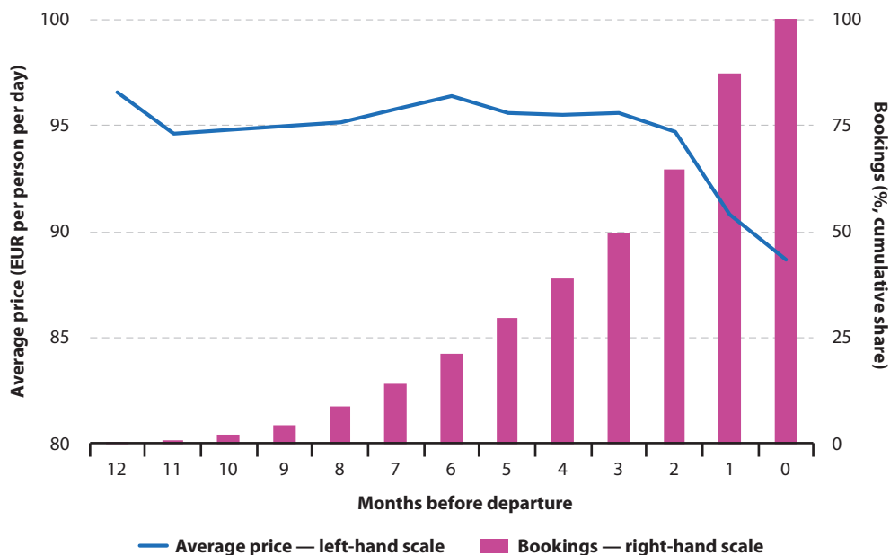
Figure 4: Bookings and average price by number of months before departure, 2013-2018
