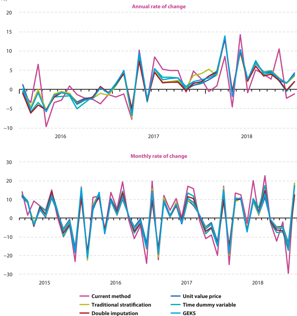
Figure 10: Comparison of transaction-based pseudo indices with the current subindex for international package holidays (ECOICOP 09.6.0.2)
