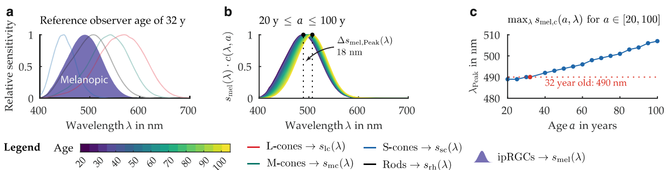
Fig. 5 Action spectrum of the ipRGCs as a function of an observer's age. (The Figure is reprinted from Zandi 2022 under CC BY-SA 4.0 license).
