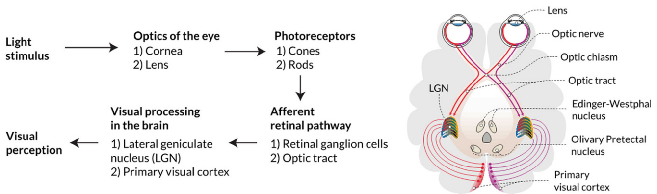
Fig. 1 Simplified processing pathway of the human's visual perception in response to light. (The Figure is reprinted from Zandi 2022 under CC BY-SA 4.0 license)
