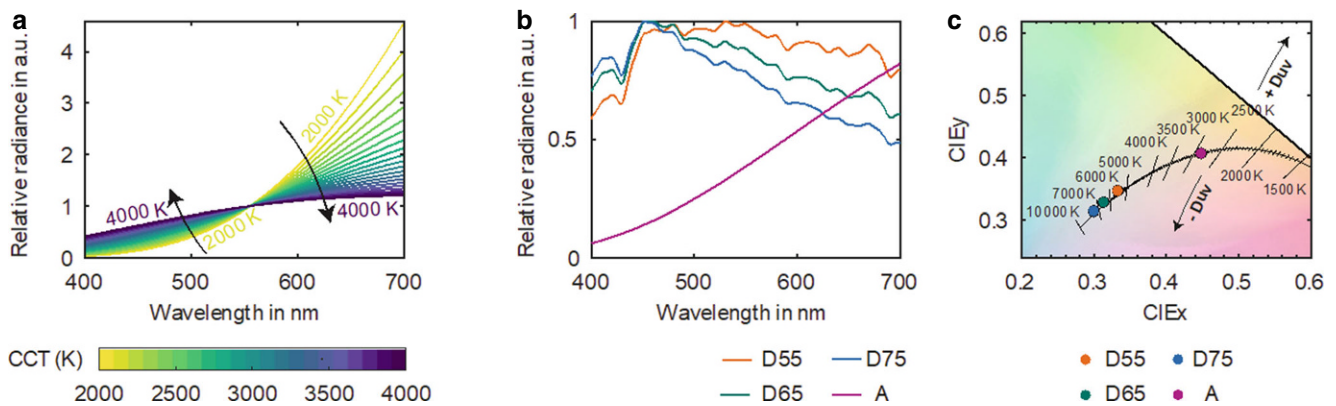
Fig. 4 Association between the spectra of the black body radiator and standard illuminants (D55, D65, D75 and A) with the Planckian locus in the CIE x -2° colour space. (The Figure is reprinted from Zandi 2022 under CC BY-SA 4.0 license)
