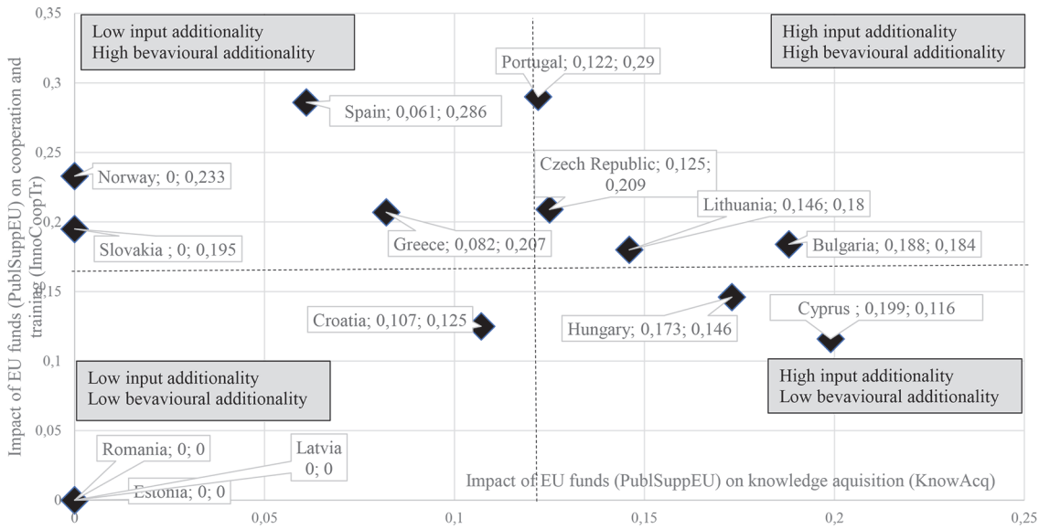
Figure 2. Results of path analysis for selected EU countries—input additionality and behavioral additionality.
