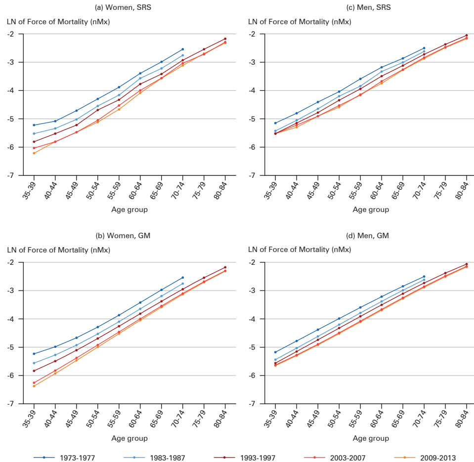
Fig. 1: Gompertz-Makeham (GM) fit for selected years for India, by sex
