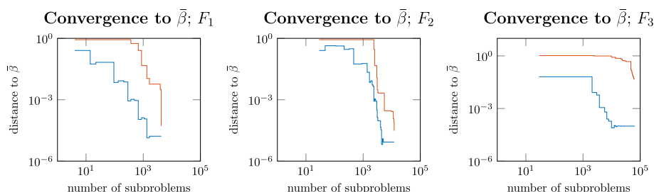
Fig. 2 Distance between the calculated solution \tilde{\beta} and the best known vertex (blue) and the furthest active vertex (red) respectively for each iteration. (Color figure online)
