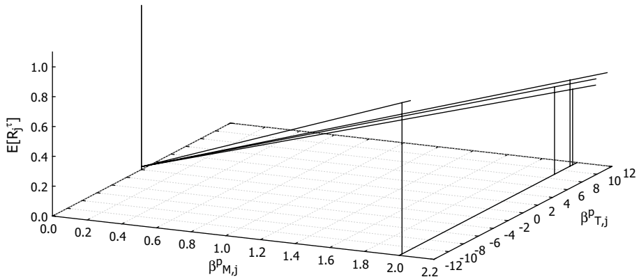
Fig. 6 Representation in pre-tax beta and after-tax expected return space. The vertical lines at \beta_{M,j}^p = 2 are there to better visualize the different heights of the different SMLs of the different assets. Source: Own depiction from numerical example in the appendix
