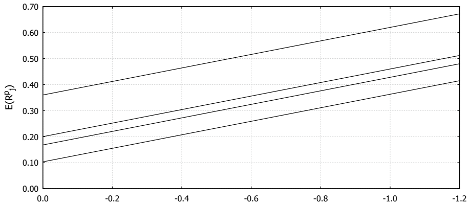
Fig. 3 Representation in pre-tax beta and pre-tax expected return space, Source: Own depiction from numerical example in the appendix
