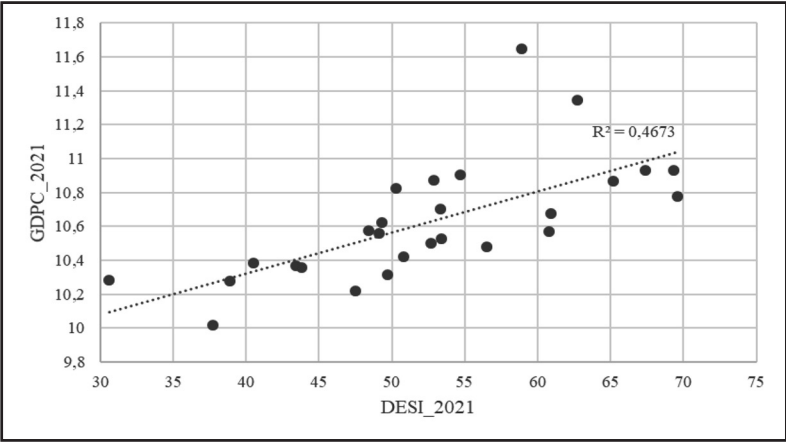
Figure 3. Regression analysis between the DESI and GDPC in 2021. Source: Own processing.
