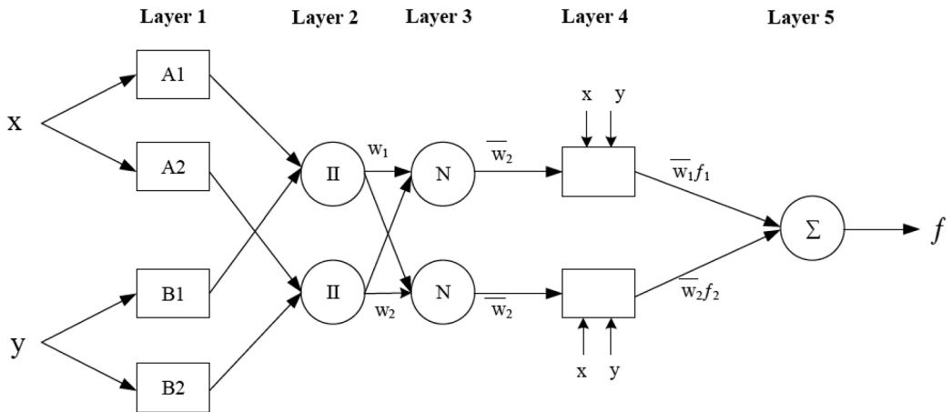
Figure. 1. Basic structure of the ANFIS. Source: Salleh et al., 2018.
