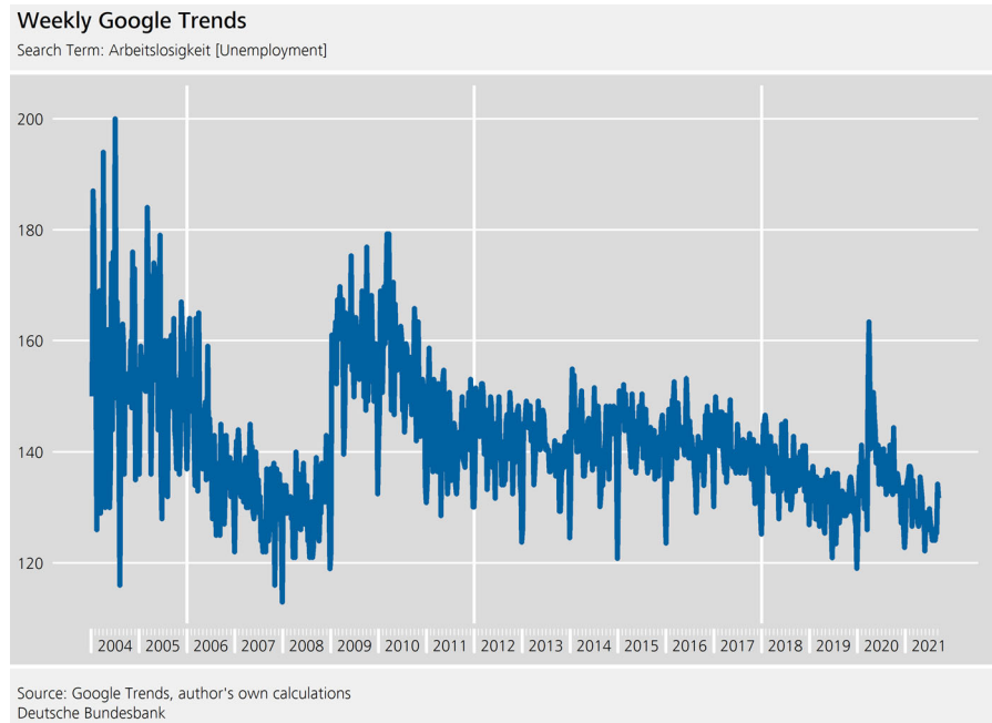
Fig. 6 Weekly Google Trends. Search Term: Arbeitslosigkeit (unemployment)
