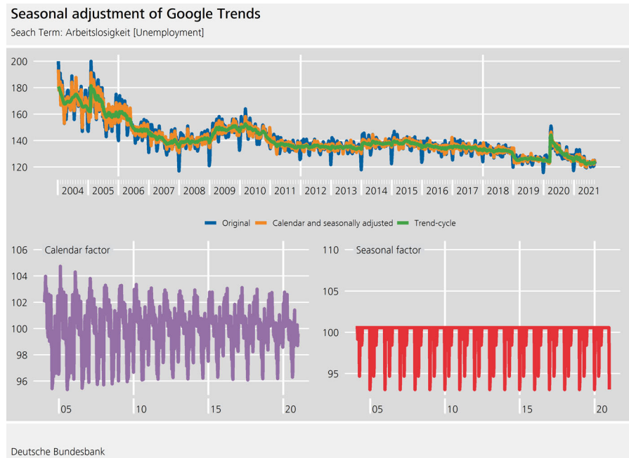
Fig. 7 Seasonal adjustment of Google Trends. Search Term: Arbeitslosigkeit (unemployment)
