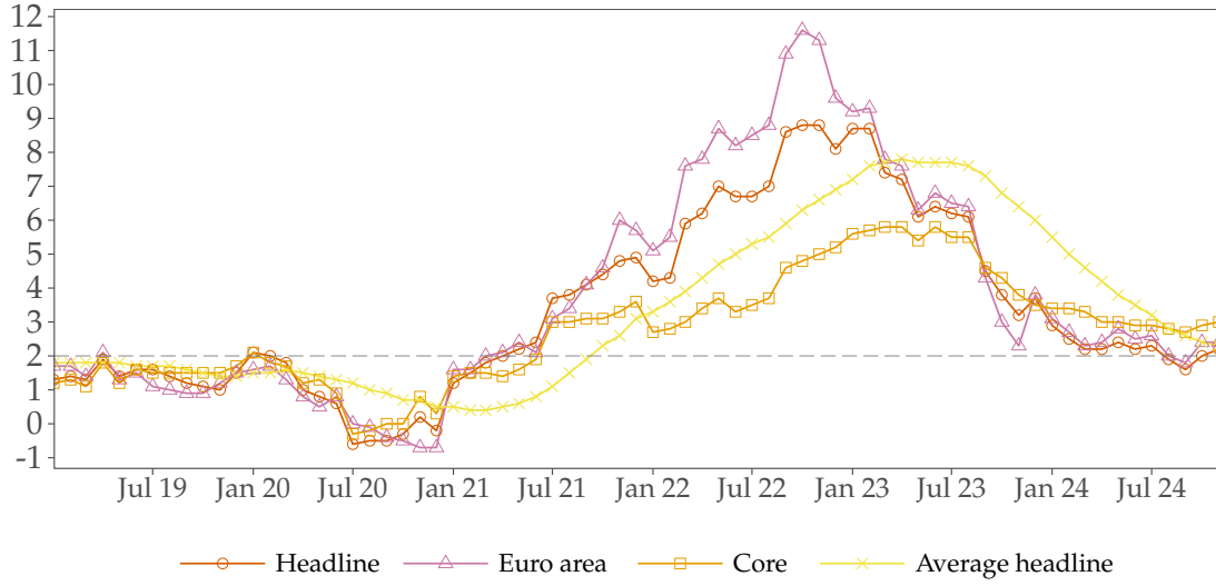
Figure 4 Inflation measures
