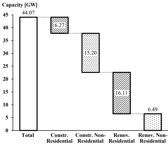
Figure 3: Computed capacity additions resulting from obligation
