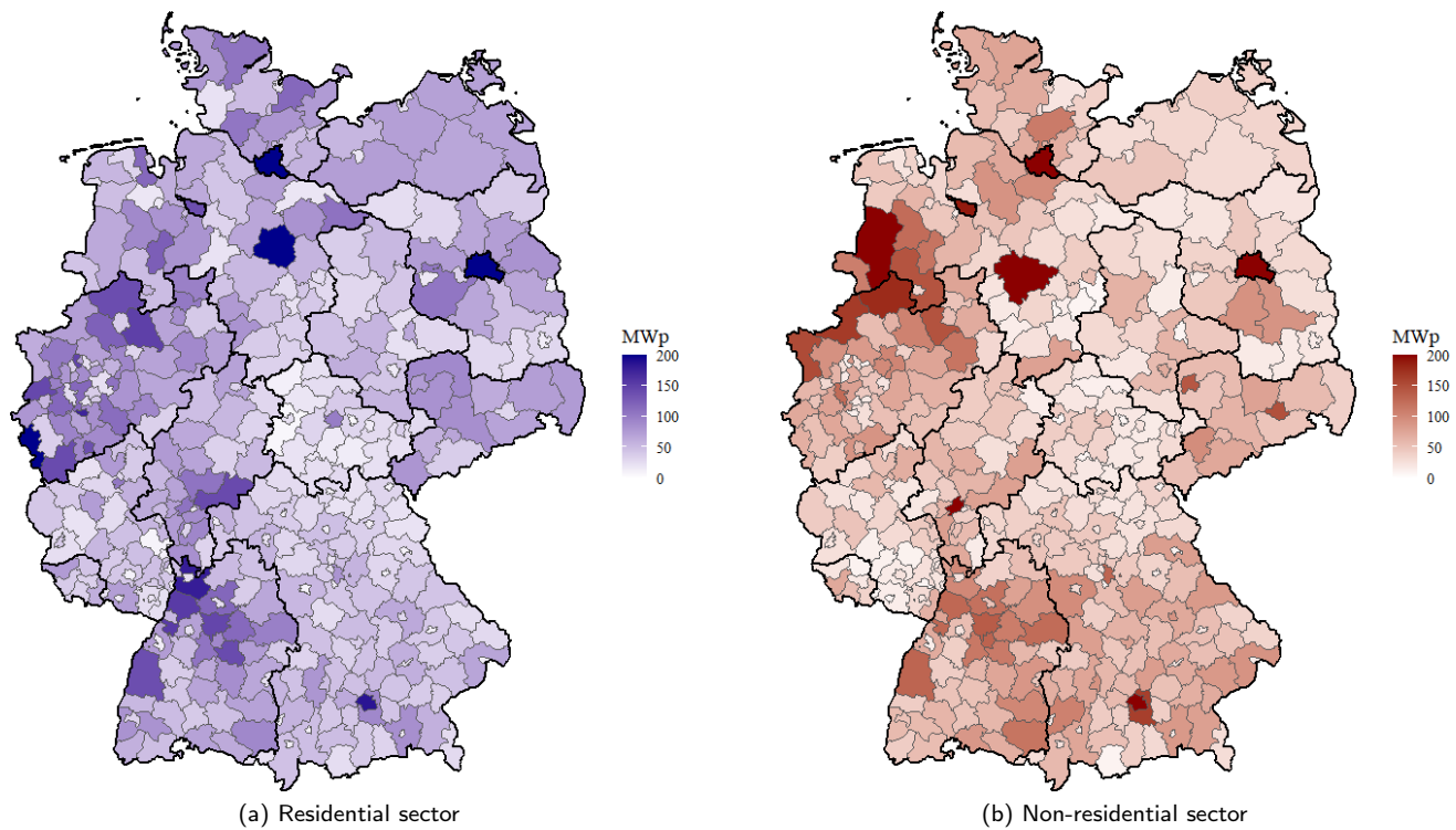
Figure 5: Cumulative PV capacity increase during 2024-2030 by an obligation combined for building construction and renovation by NUTS3 region
