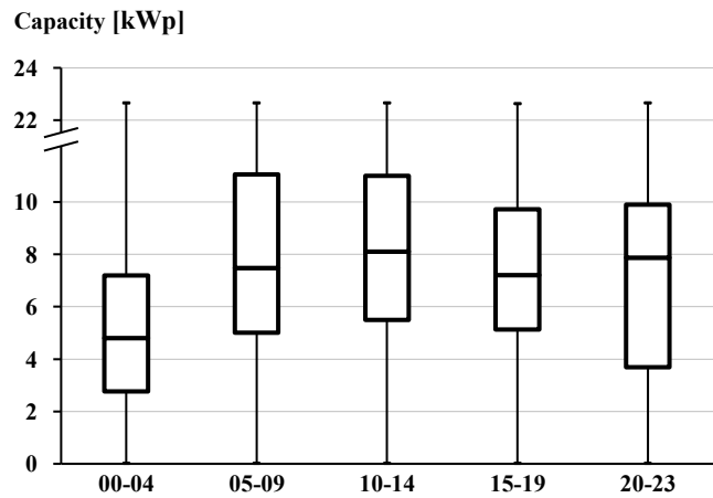
Figure 1: Distribution of observed residential PV capacity additions
