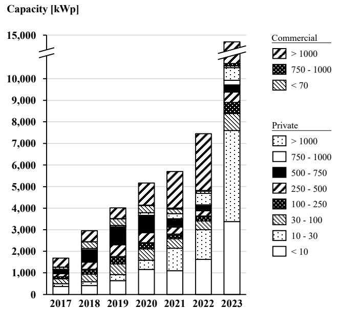
Figure 7: Annual Net Additions by Size Categories
