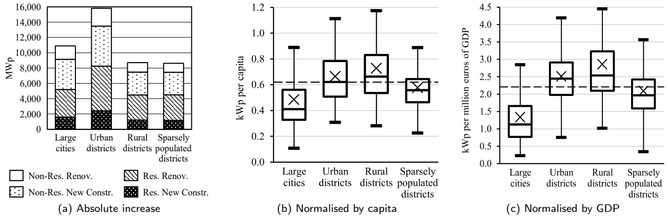
Figure 6: Cumulative PV capacity increase during 2024-2030 by an obligation combined for building construction and renovation by settlement structure
