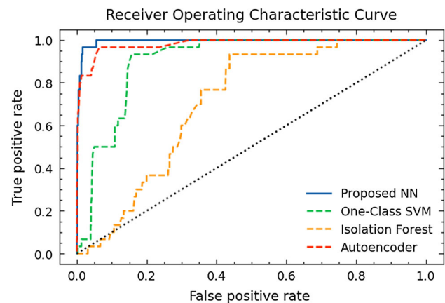
Fig. 5 Receiver operating characteristic for the trained network using verified false states. An Autoencoder, One-Class SVM, and Isolation Forest are used for benchmarking
