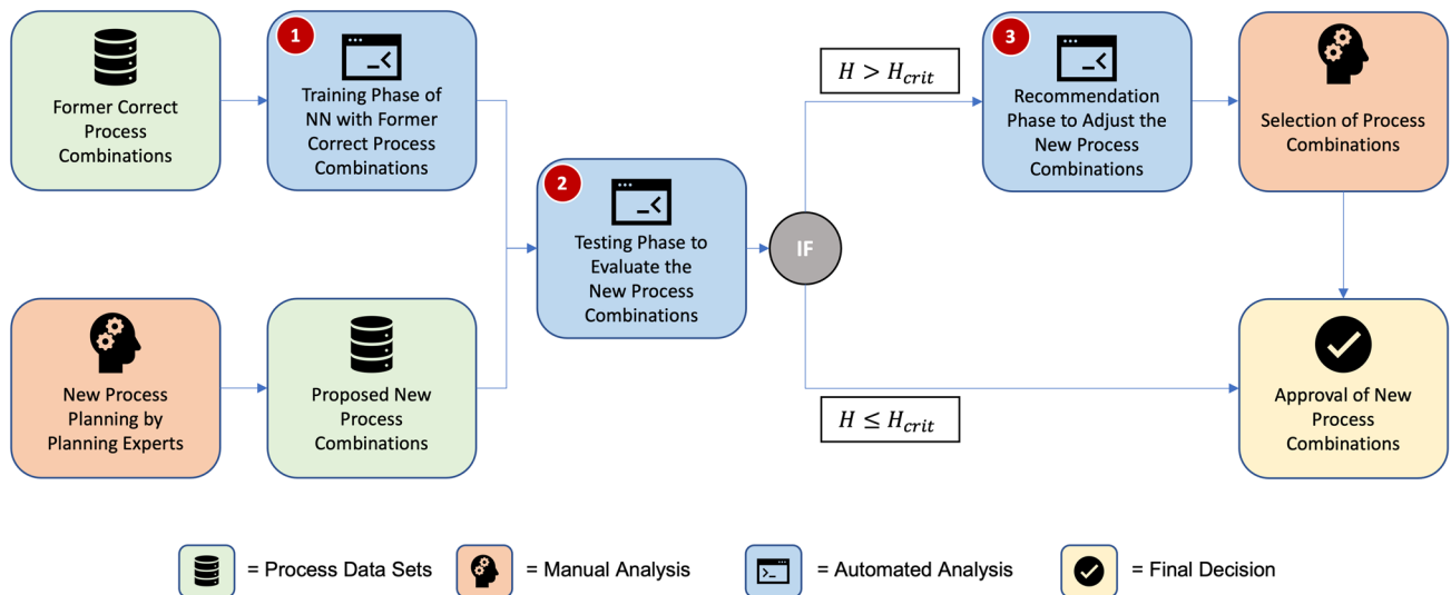
Fig. 2 Sketch of the applied concept for usage and implementation in manufacturing of the proposed NN during PP by a planning expert
