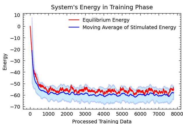
Fig. 3 Equilibrium and stimulated state's energy during training phase. The moving average of the stimulated states is calculated per 100 training data. The blue shaded region is the 3- \sigma region of the moving average
