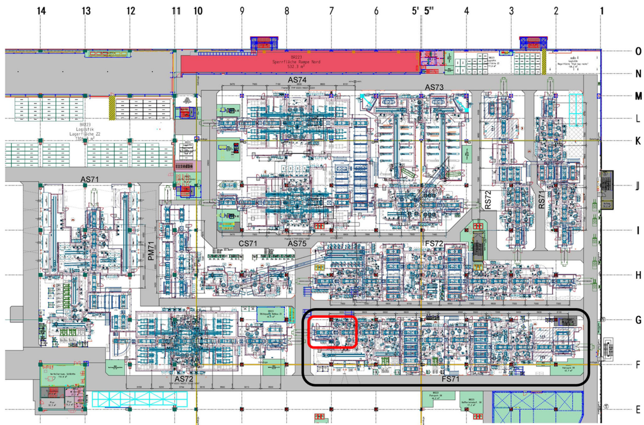
Fig. 7 Plant layout of the assembly of the side panels of one location. All here visible working stations and cells are applied in the analysis. The manufacturing line FS71 is located in the lower right of the map. The exemplary process combination is located at the manufacturing cell marked in red
