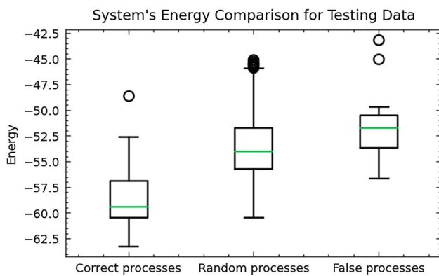
Fig. 4 Median energy levels per state of validated correct process combinations, random combinations, and validated incorrect combinations. The boxes show the lower to upper quartile. The median is marked with a line. The whiskers indicate the 1.5 times interquartile range above/below the quartile. Data outside of the whiskers are marked as dots
