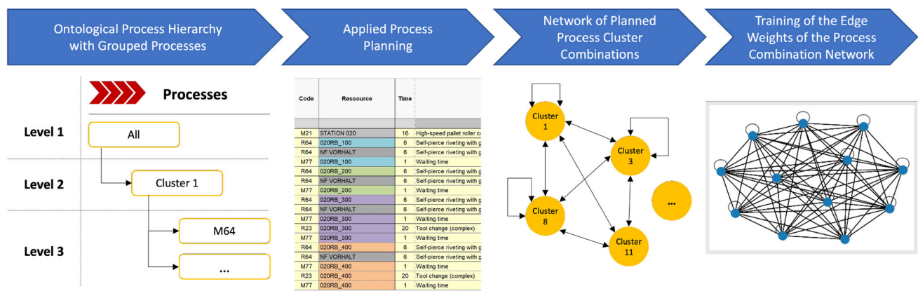
Fig. 1 The proposed methodology follows four consecutive steps: 1. similar processes are grouped in clusters, 2. process planners design a valid process combination, 3. the process combination is translated into a combination network, 4. the network's edge weights representing the likelihood of a process combination are trained
