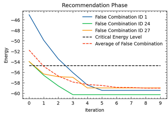
Fig. 6 Energy level after multiple iterations of recommendation with single activations or deactivations of processes per iterative step
