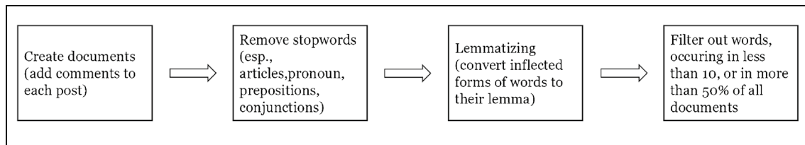
Fig. 1 LDA preprocessing steps
