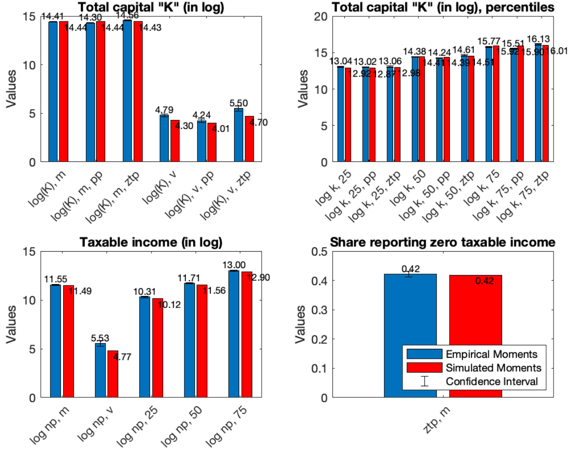
Figure 4: Model fit
