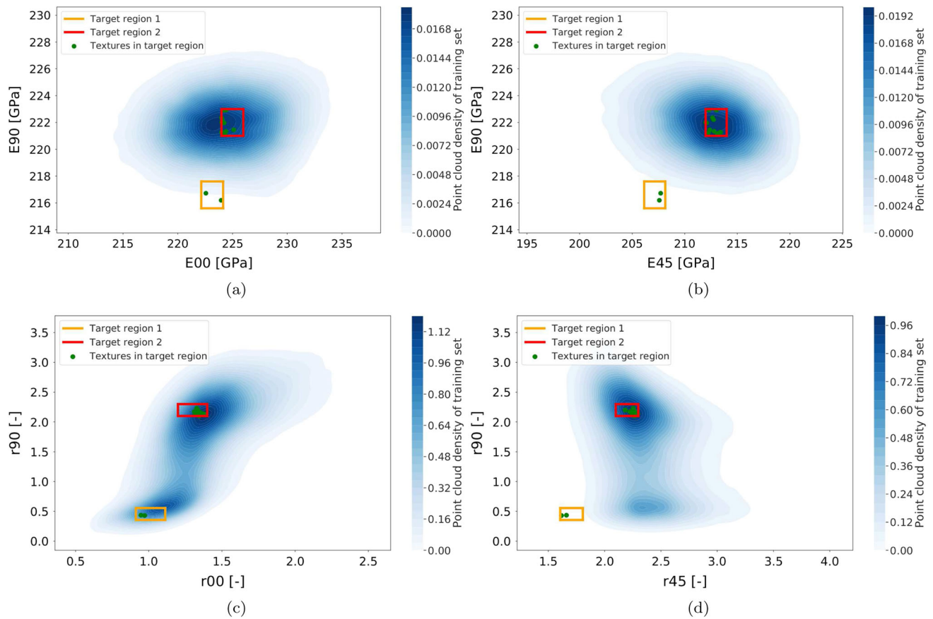
Fig. 8 Density of the training set projected on different planes of the property space: the Young's modulus at a 0 vs. 90 degree and b 45 vs. 90 degree for the r -values at c 0 vs. 90 degree and d 45 vs. 90 to rolling
