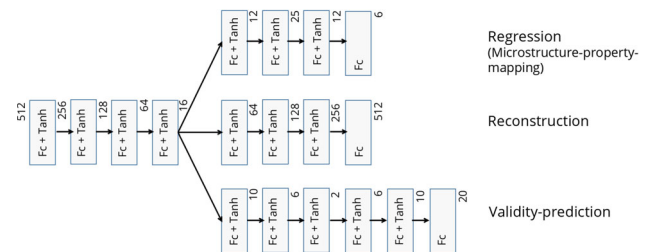
Fig. 6 One twin part of the SMTL model with the annotation of the dimension size of the layers. Fc denotes fully-connected layers and \tanh denotes hyperbolic tangent activation function
