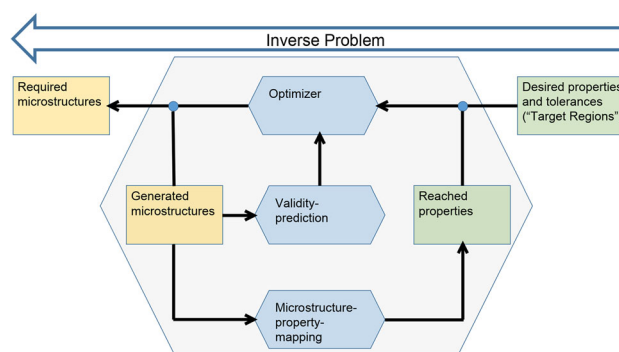
Fig. 1 General concept of the MTL-based optimization approach to solve materials design problems
