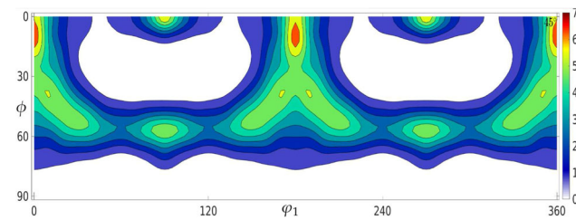
Fig. 5 \varphi_2 = 45^\circ section of the orientation distribution function to visualize the \gamma -fiber of the cold rolled DC04 steel texture
