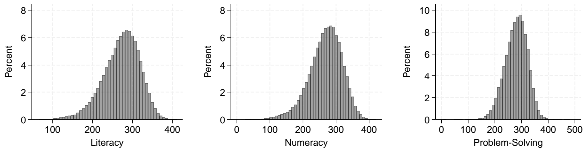
Figure 3: Skill scores
