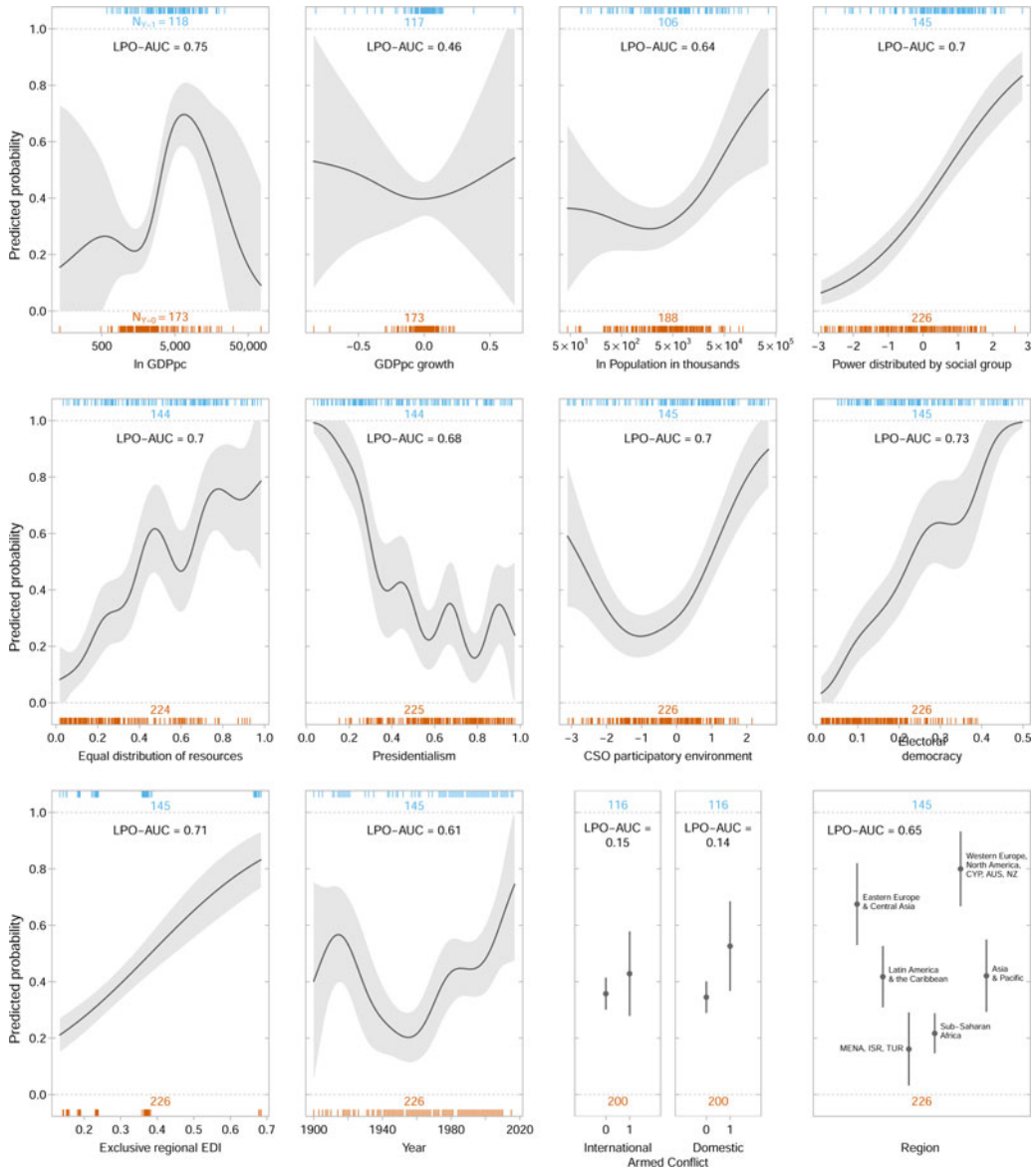
Figure 7. Predicted probabilities of episode success under 13 bivariate models. Ridge-penalized random-effect smoothing for exclusive regional EDI, Gaussian process models for all other non-binary covariates. 95 percent confidence intervals and regions. All covariates are at their pre-episode values. One episode (Croatia, starting in 1992) is excluded from the GDPpc growth model due to an extremely outlying value.
