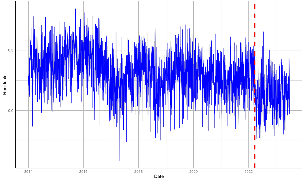
Figure 5: Residuals.
