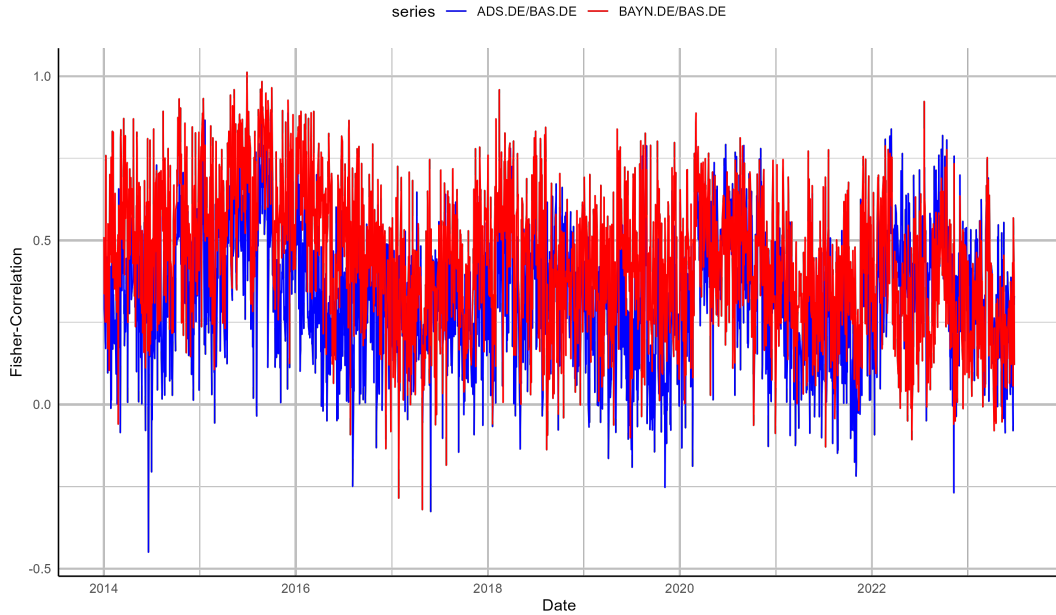
Figure 4: Realized correlations.
