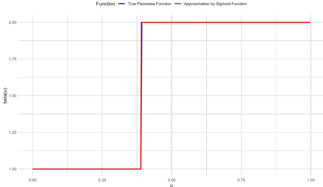
Figure 1: Approximation of (21) with Sigmoid Function.
