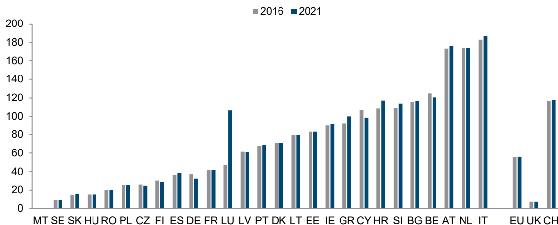
Figure 13 / Length of low-voltage circuits \leq 220 kV, in km per 1,000 km 2 of surface area
