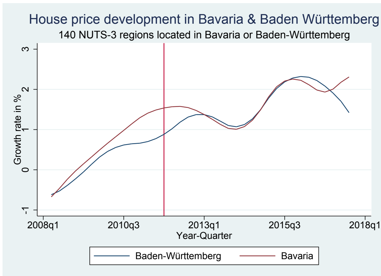
Figure A.2: Quarterly HPI growth rate of all regions in Baden Württemberg and Bavaria
