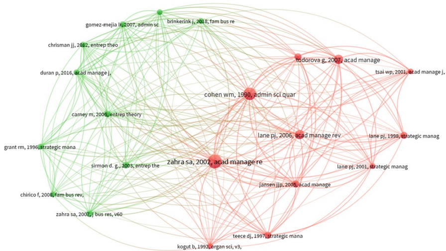
Fig.3 Co-citation analysis
