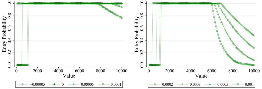
Figure 2: Partial-entry equilibrium z for Each CARA Parameter r . Note: The premium is \pi = 991 . The entry probability is 1 - z(v) . The equilibrium for r = 0 is the minimal-entry equilibrium z^d in Theorem 3 (ii) with the cutoff v^d = 600 .
