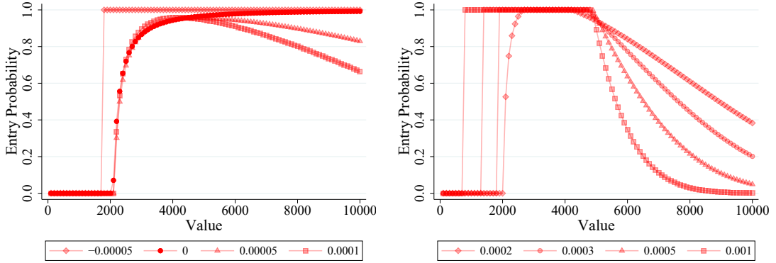
Figure 1: Partial-entry equilibrium z for Each CARA Parameter r . Note: The premium is \pi = 1 . The entry probability is 1 - z(v) . The equilibrium for r = 0 is the minimal-entry equilibrium z^c in Theorem 3 (i) with the cutoff v^c = 2100 .
