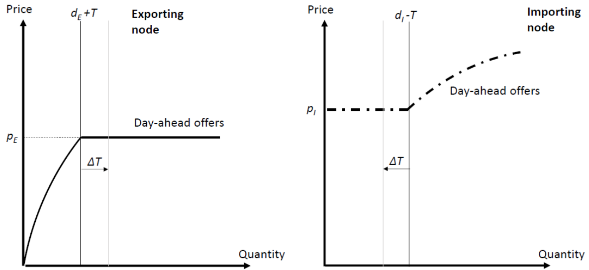
Figure 3: The equilibrium in a day-ahead market with two nodes/zones, where the cross-zonal transmission capacity between the two nodes has been exaggerated by \Delta T .
