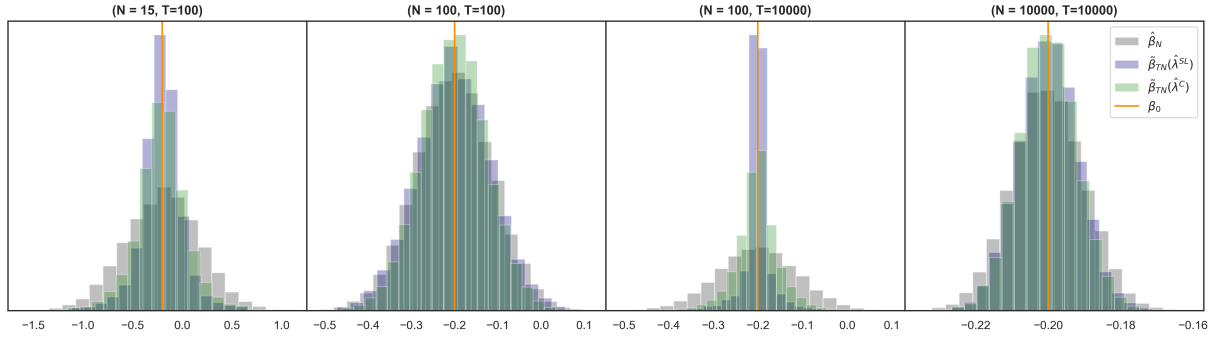
Figure 2: Distributions of \hat{\beta}_N , \tilde{\beta}_{NT}(\hat{\lambda}^{SL}) and \tilde{\beta}_{NT}(\hat{\lambda}^C) for exogenous observational data.
