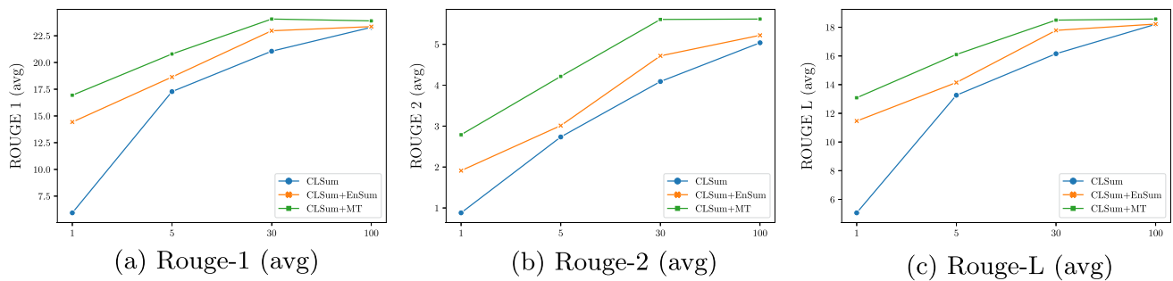
Fig. 6 Few-shot results without (CLSum) and with intermediate task (+EnSum) and cross-lingual fine-tuning (+MT) for different sizes of the training data in the target language (i.e., different number of shots ): 1%, 5%, 30% and 100% of the X-SCITLDR training set of each target language
