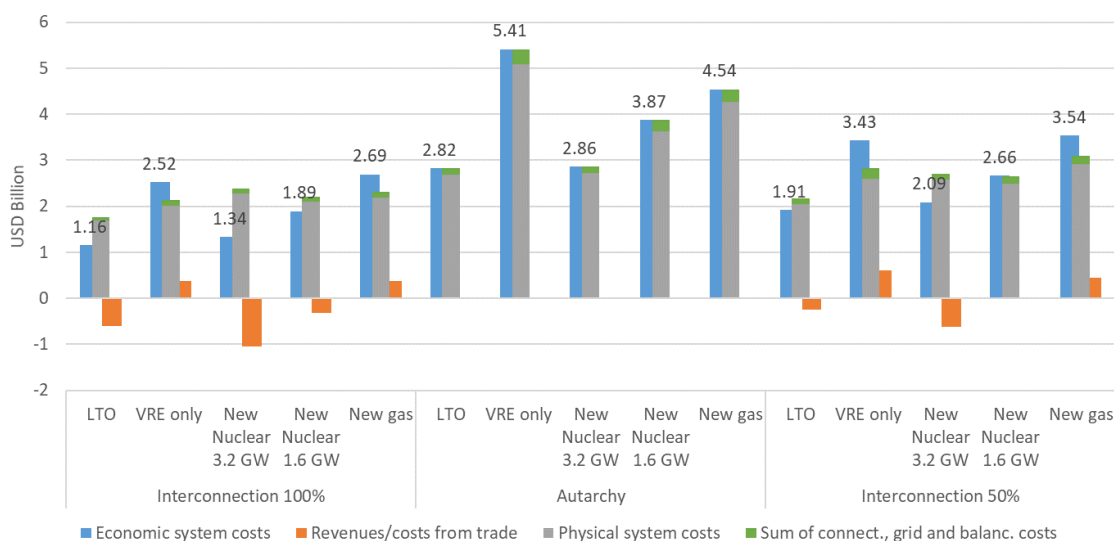
Figure 2: System costs of different scenarios to reach net zero carbon emissions in Switzerland (billion USD per year)
