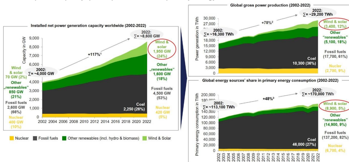
Figure 1: Global power capacity, power production, and primary energy
