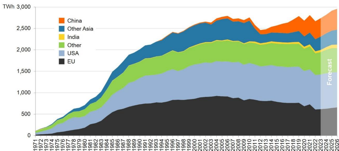
Figure 2: Global nuclear power generation
