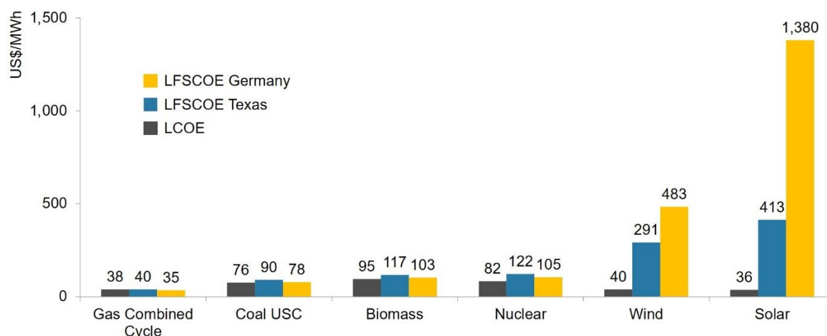
Figure 3: Full system cost of nuclear vs alternatives
