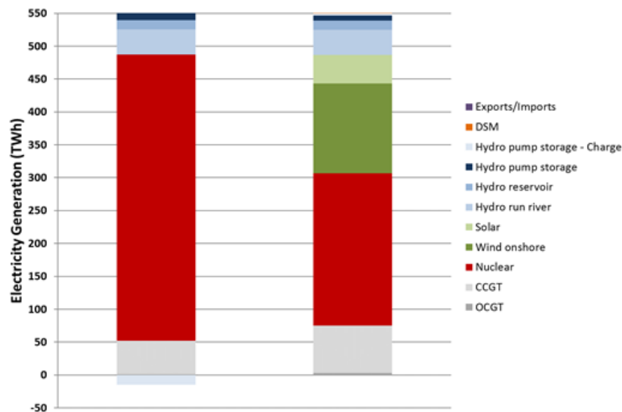
Figure 3: The trade-off between plant-level generation costs and system costs
