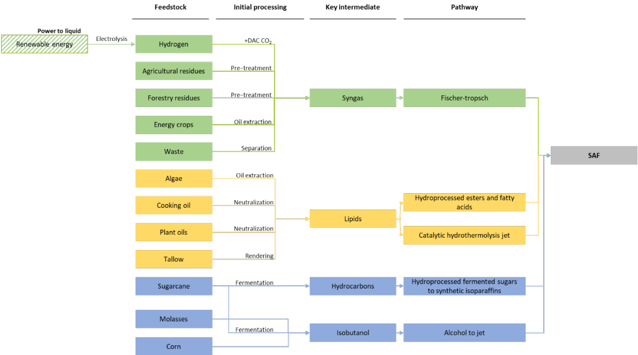
Figure 2: Methods for SAF production
