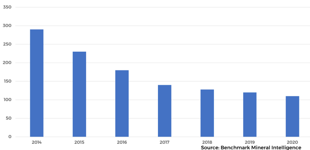
Lithium ion cell price, Large contract, Automotive, $/kWh
