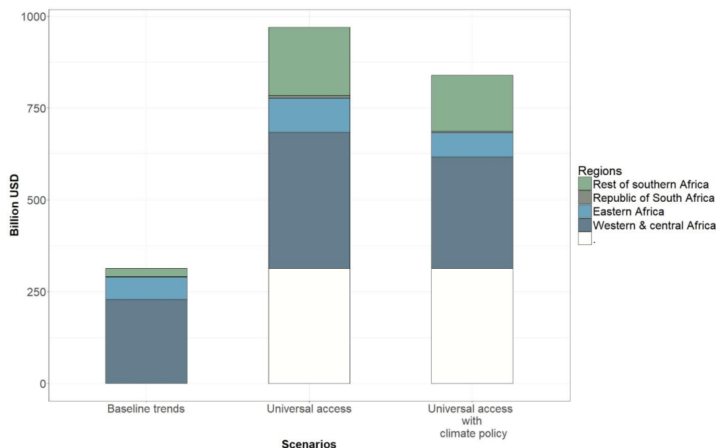
Additional investments for universal electricity access compared to the baseline trend, 2010–2030
