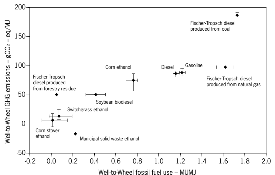
Figure1: Life cycle Fossil Fuel Use and GHG Emissions per MJ Fuel for Biofuels and Synthetic fuels in the USA
