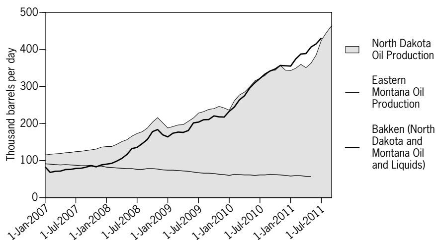
Figure 4: North Dakota, Montana, and Bakken Oil Production
