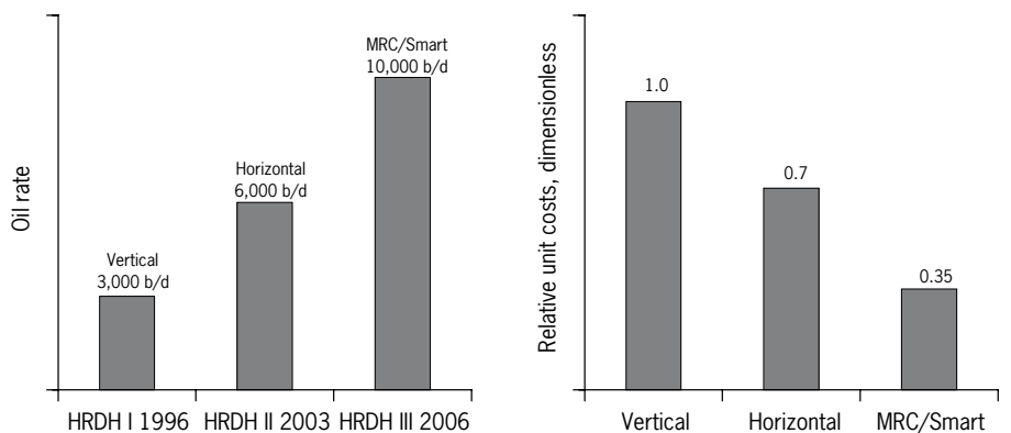
Figure 1: Relative Unit Well Costs and Oil Rates for Haradh-III
