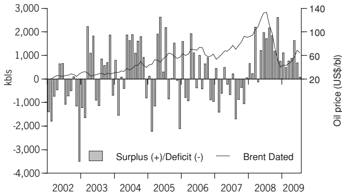
Figure 1: Oil Supply/Demand Balance with Respect to Oil Price
