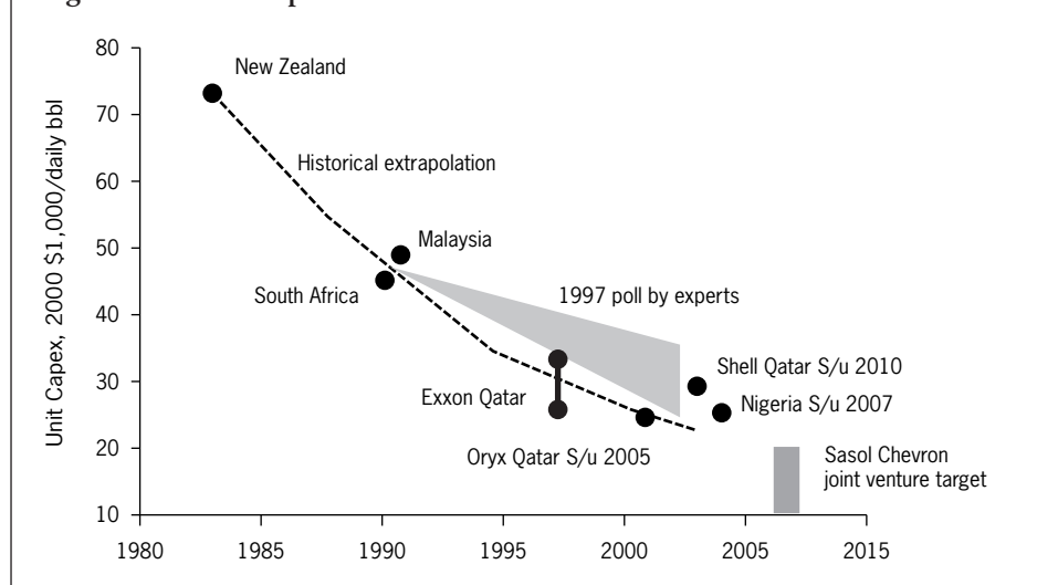
Figure 1: GTL Capital Costs – Trend
