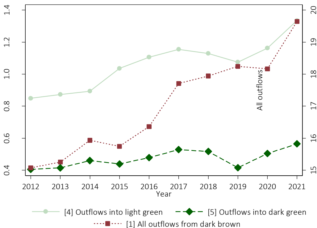
Figure 6: Outflow rates from brown occupations (in %)
