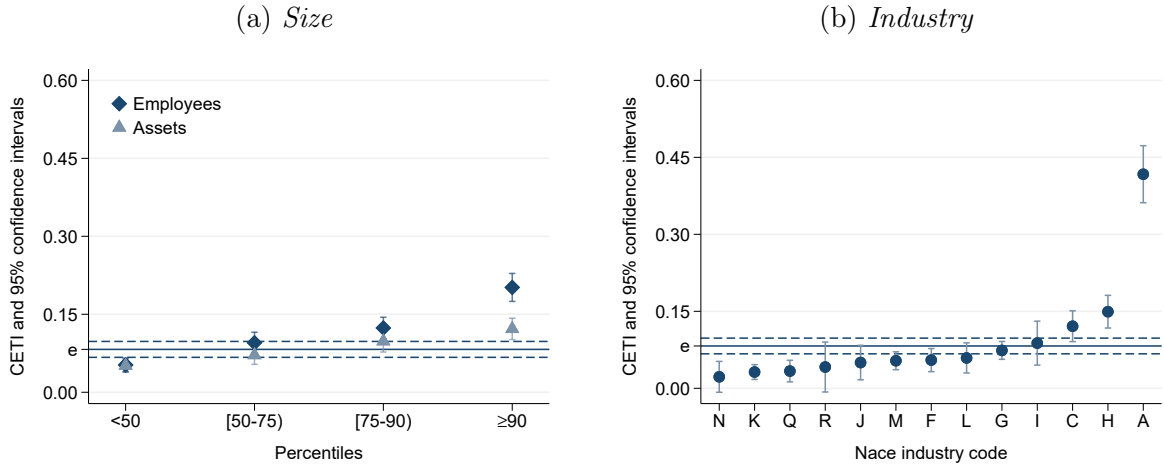
Figure 4 – Bunching at the €200,000 threshold: Firms' heterogeneity
