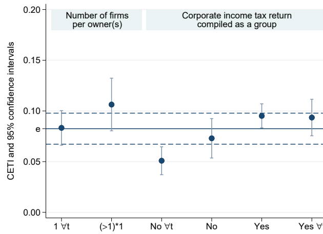
Figure A4 – Bunching at the €200,000 threshold: Extensive margin response
