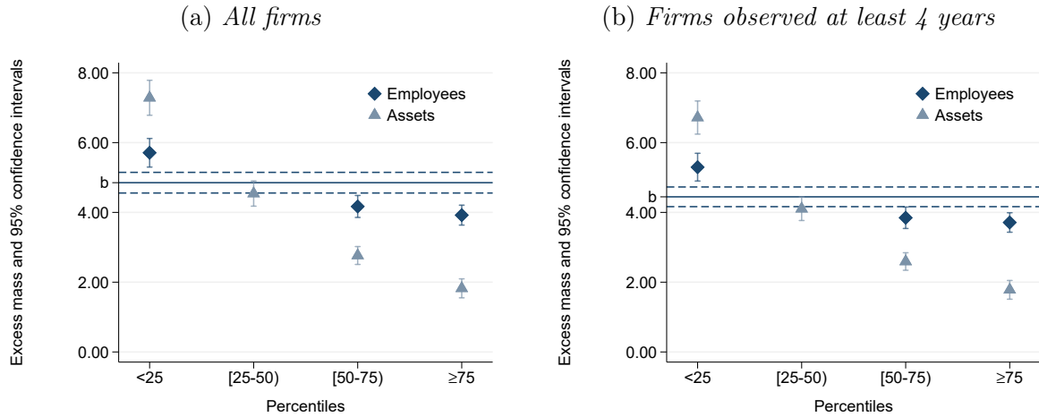
Figure A25 – Bunching at the zero threshold: Heterogeneity in firms' size
