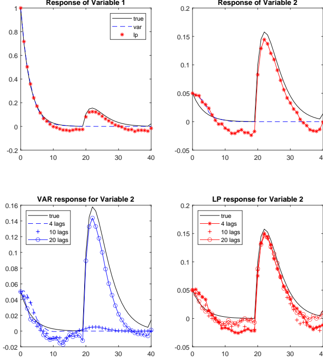
Figure C.1: Monte-Carlo results
