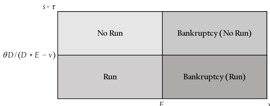
Figure 1: Possible Equilibria
