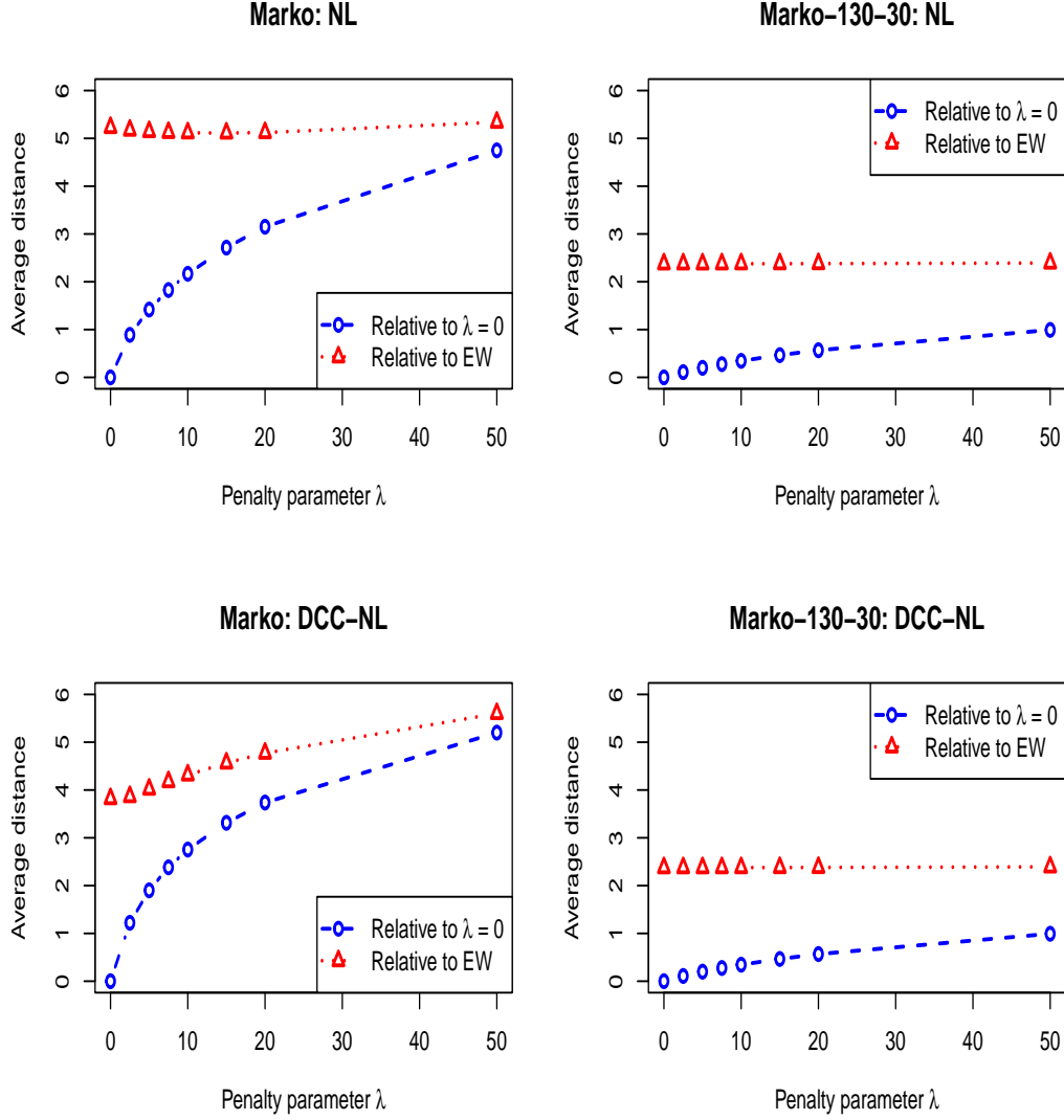
Figure 4.2: Average-distance measure (4.2) as a function of the penalty parameter \lambda relative to two reference portfolios. These graphs are for the four Marko-type portfolio formulations.
