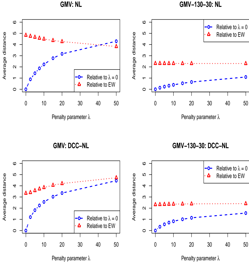
Figure 4.1: Average-distance measure (4.2) as a function of the penalty parameter \lambda relative to two reference portfolios. These graphs are for the four GMV-type portfolio formulations.
