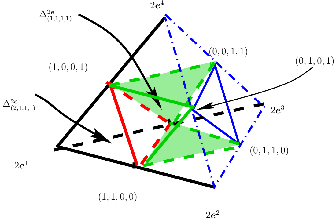
Figure 2.3: The octahedron \Delta_{1111}^2
