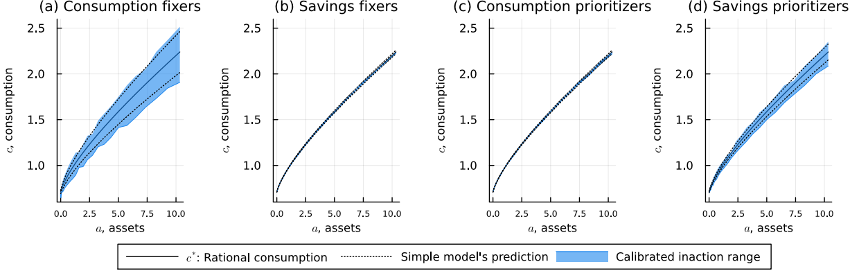
Figure 6: Inaction regions in the calibrated quick-fixing model
