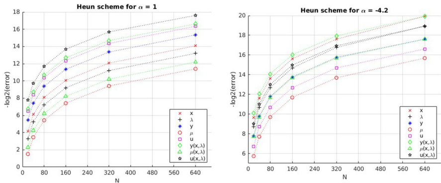
Fig. 1 Errors for the Heun scheme with the values \alpha = 1 and \alpha = -4.2
