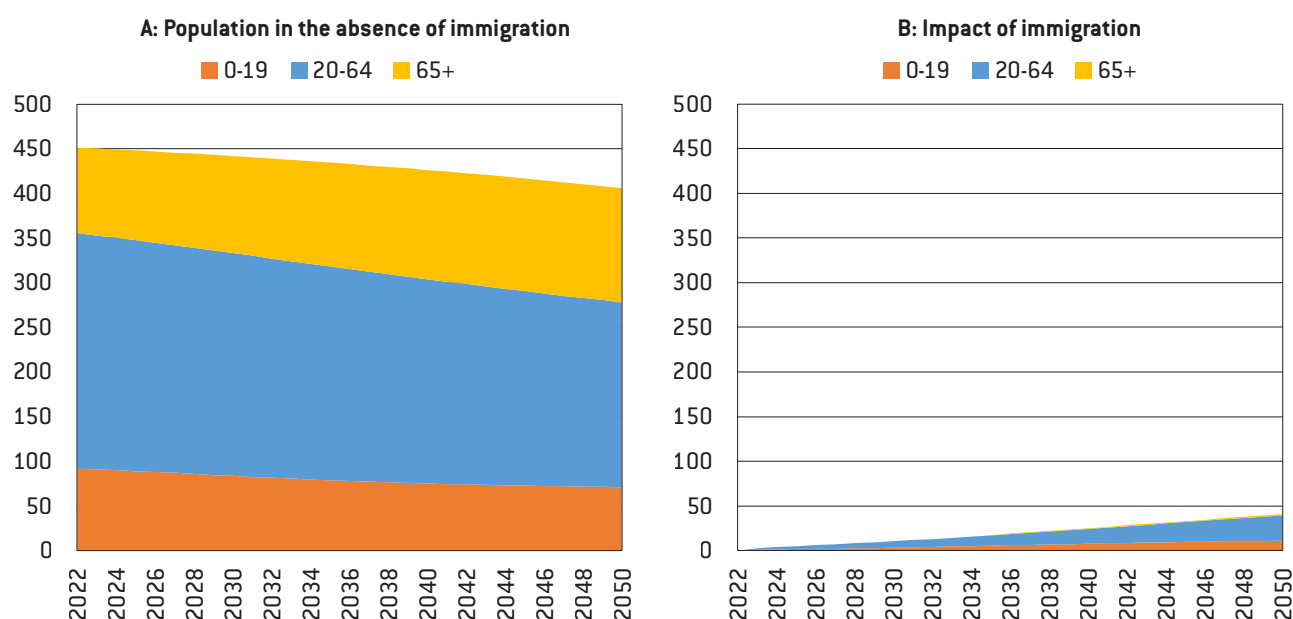
Figure 1: Baseline population projections for the EU
