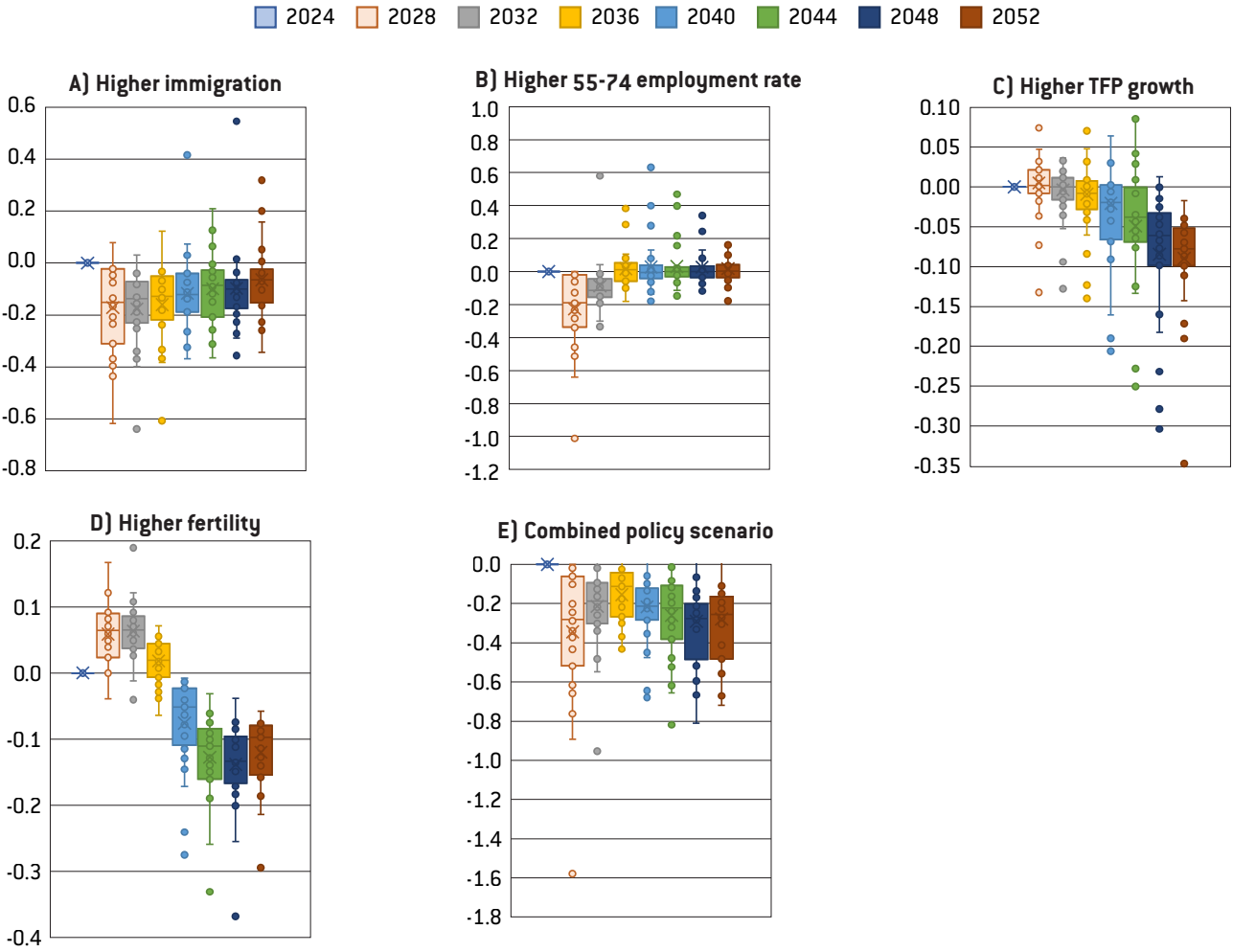
Figure A3 (referring to Figure 7): Difference between structural primary balances required under scenarios presumed to lower to debt sustainability risks and under the baseline, 4-year adjustment periods (% GDP)
