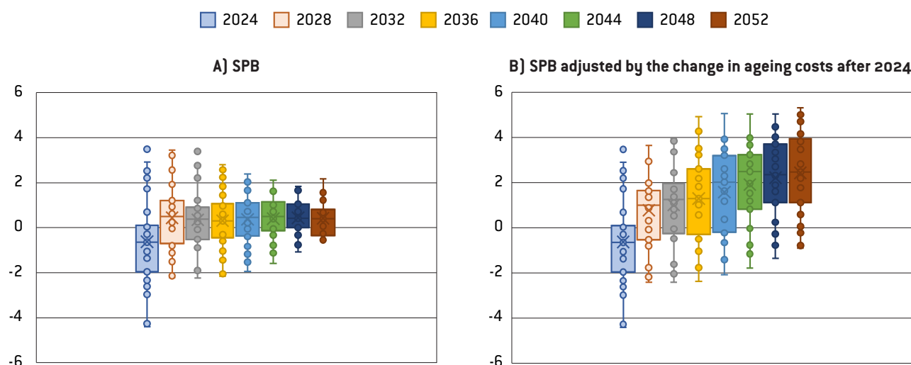
Figure A1 (referring to Figure 3): Baseline fiscal balance paths to meet EU DSA requirements and maintain the deficit below 3% of GDP, 4-year adjustment periods (structural primary balance, % of GDP)
