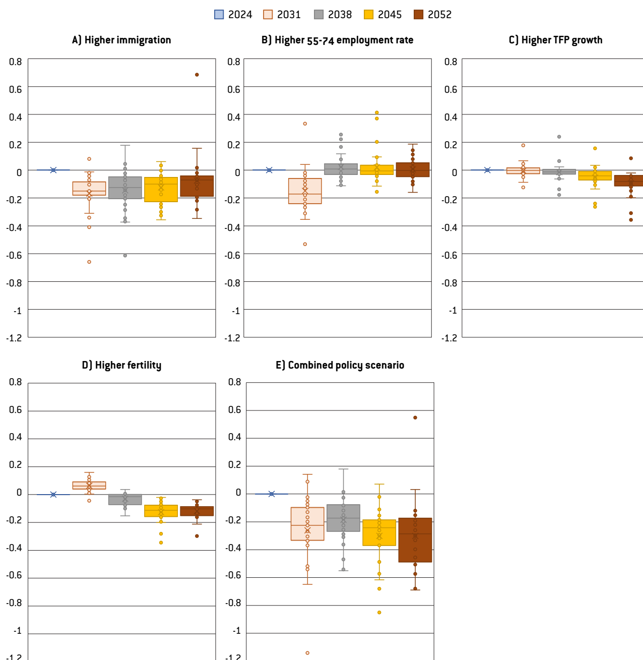
Figure 7: Difference between SPBs required under scenarios presumed to lower debt sustainability risks and under the baseline, 7-year adjustment periods (% GDP)
