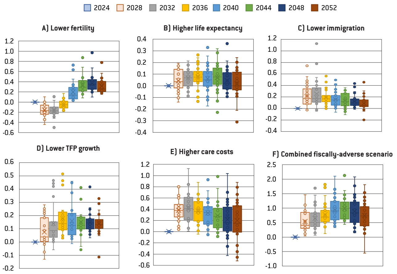
Figure A2 (referring to Figure 5): Difference between structural primary balances required under under scenarios leading to higher debt sustainability risks and the baseline, 4-year adjustment periods (% GDP)
